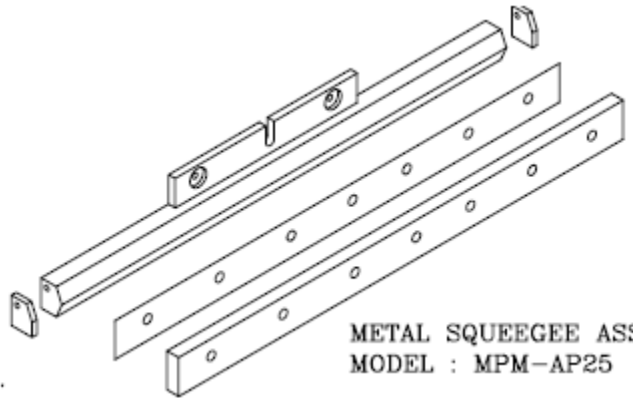
RUBBER SQUEEGEE ASSY. MODEL : DEK-249
